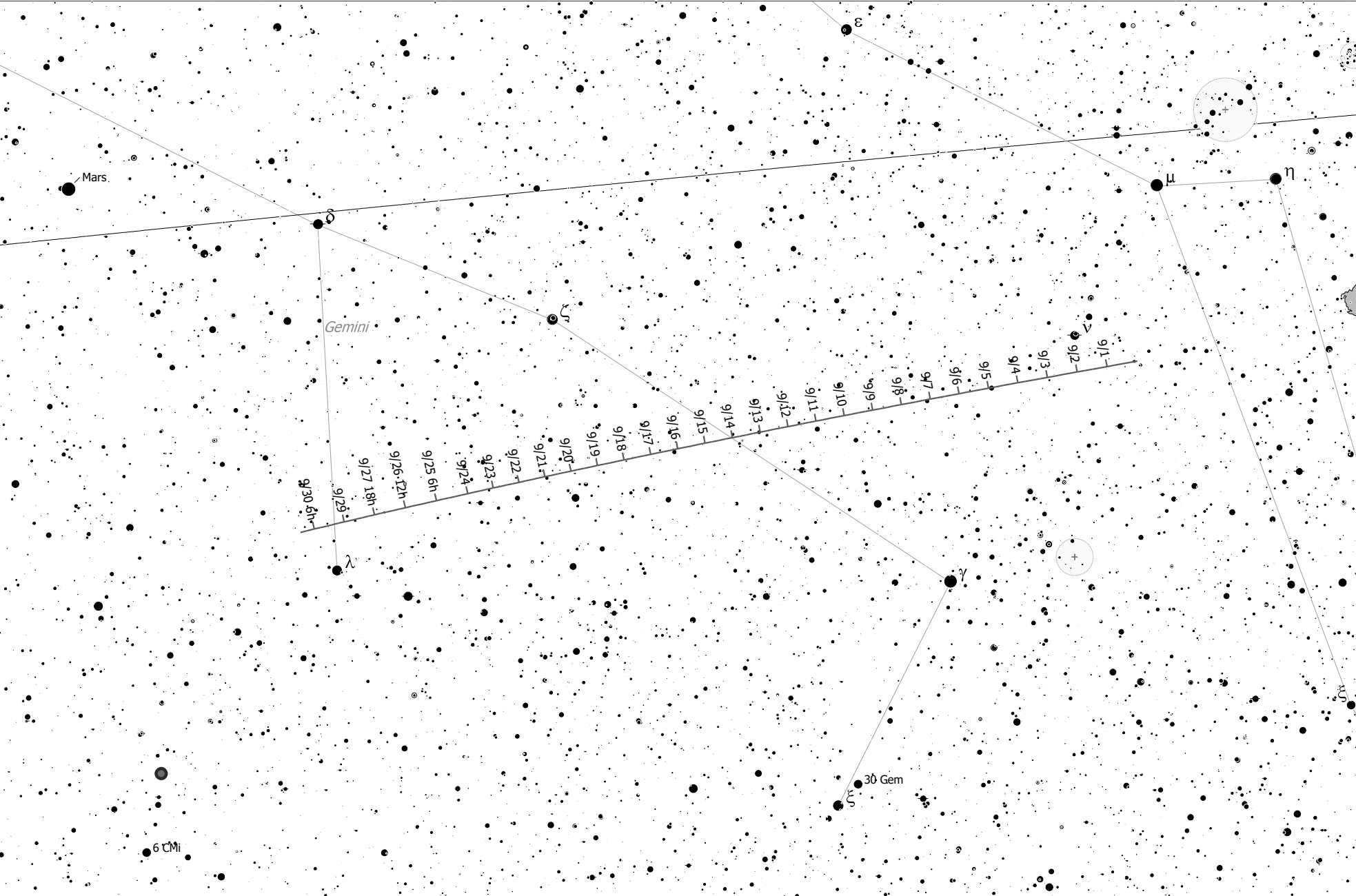
78P/Gehrels (Comet) Magnitude: 14.61 Coma Diameter: 37" SBr: 22.2 Mag/arcsec 2 Earth Distance: 2.2 AU
