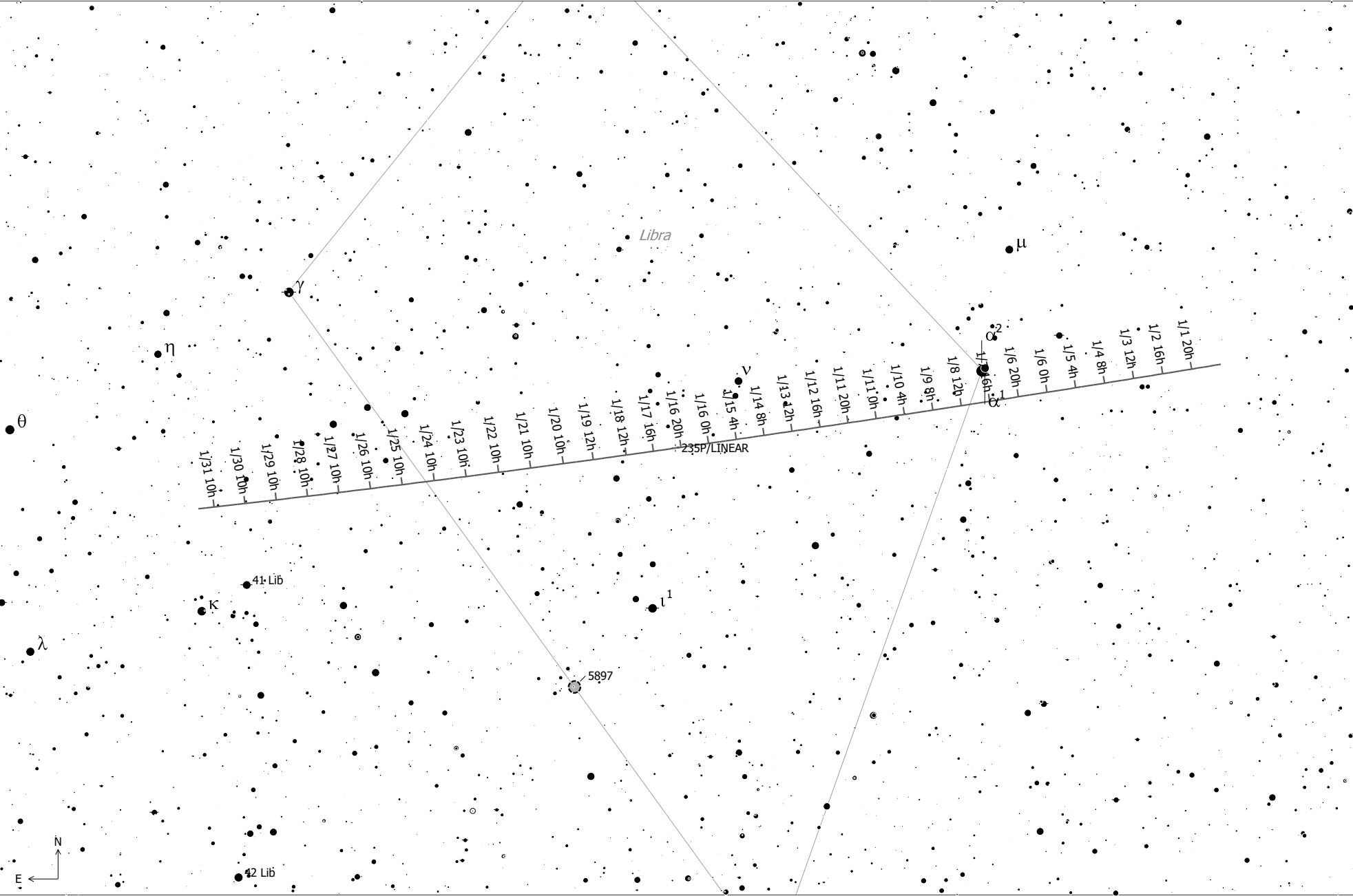
235P/LINEAR (Comet) Magnitude: 13.06 Coma Diameter: 1.1' SBr: 21.8 Mag/arcsec² Earth Distance: 2.2 AU
