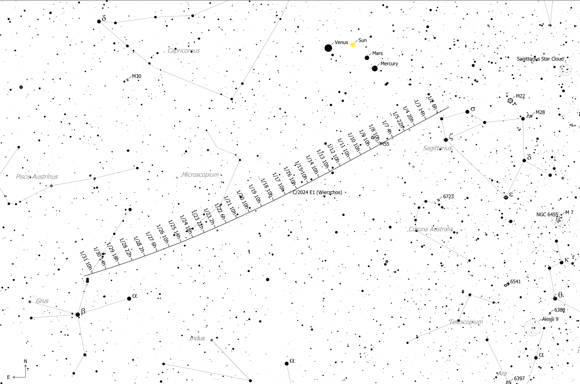
C/2024 E1 (Wierzechos) (Comet) Magnitude: 8.65 Coma Diameter: 1.8' SBr: 18.5 Mag/arcsec² Earth Distance: 1.4 AU
